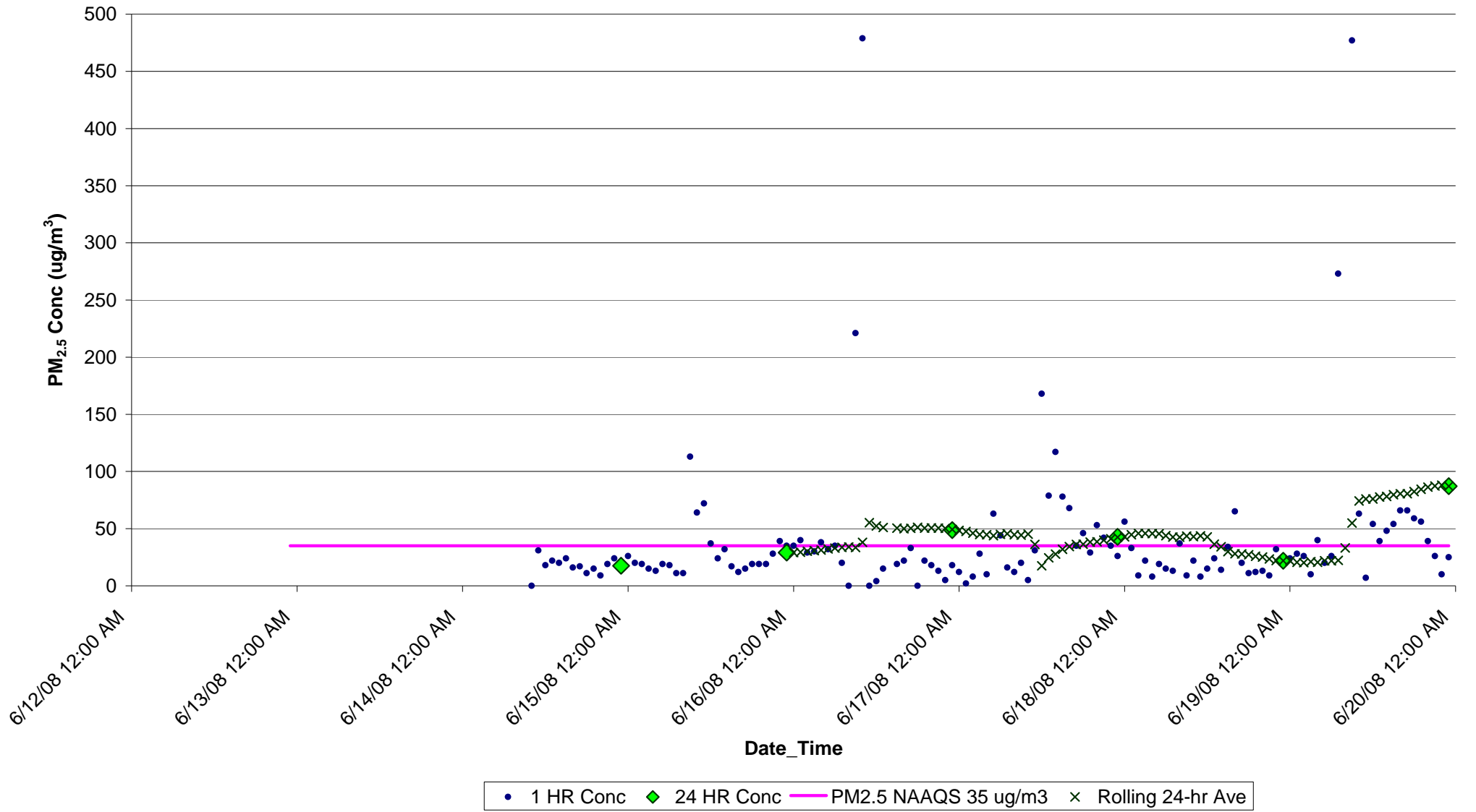
Figure F15. PM 2.5 Concentrations (ug/m 3 ) from June 12-19, 2008 for Fairfield, NC EBAM Monitor
