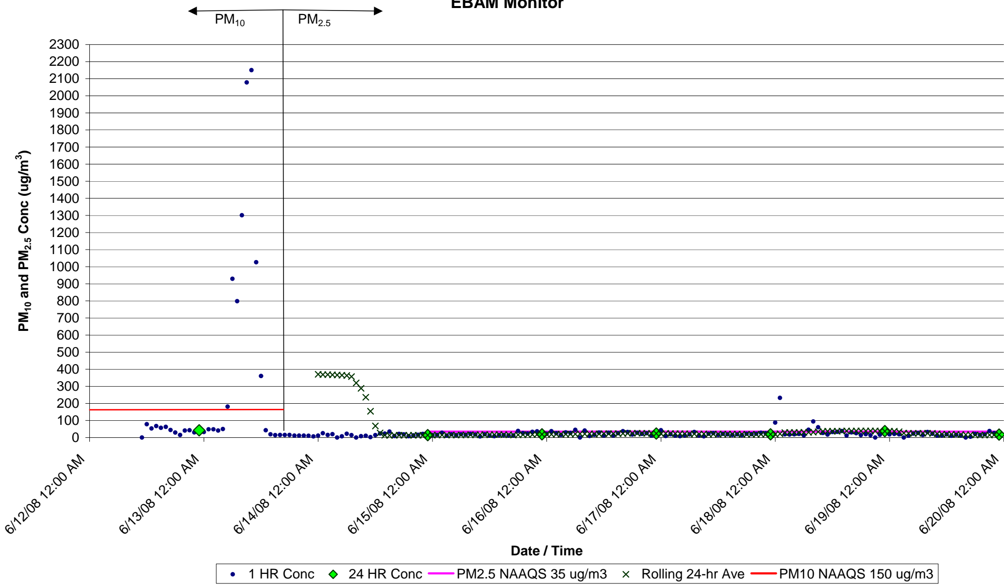
Figure F1. PM 10 and PM 2.5 Concentrations (ug/m 3 ) for June 12-19, 2008 at Belhaven, NC EBAM Monitor
