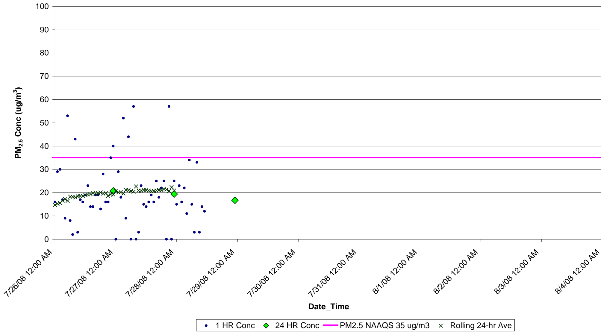
Figure F35. PM 2.5 Concentration (ug/m 3 ) from July 26-Aug 4, 2008 for Plymouth, NC EBAM Monitor
