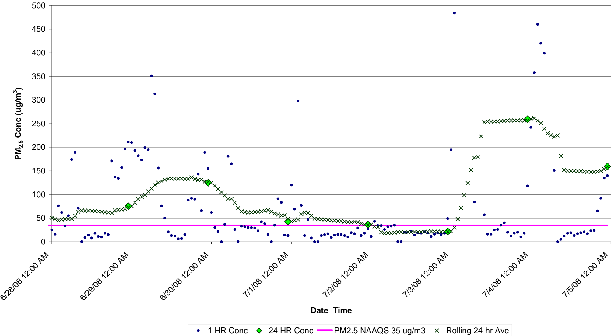
Figure F10. PM 2.5 Concentrations (ug/m 3 ) for June 28-July 4, 2008 at Columbia, NC EBAM Monitor
