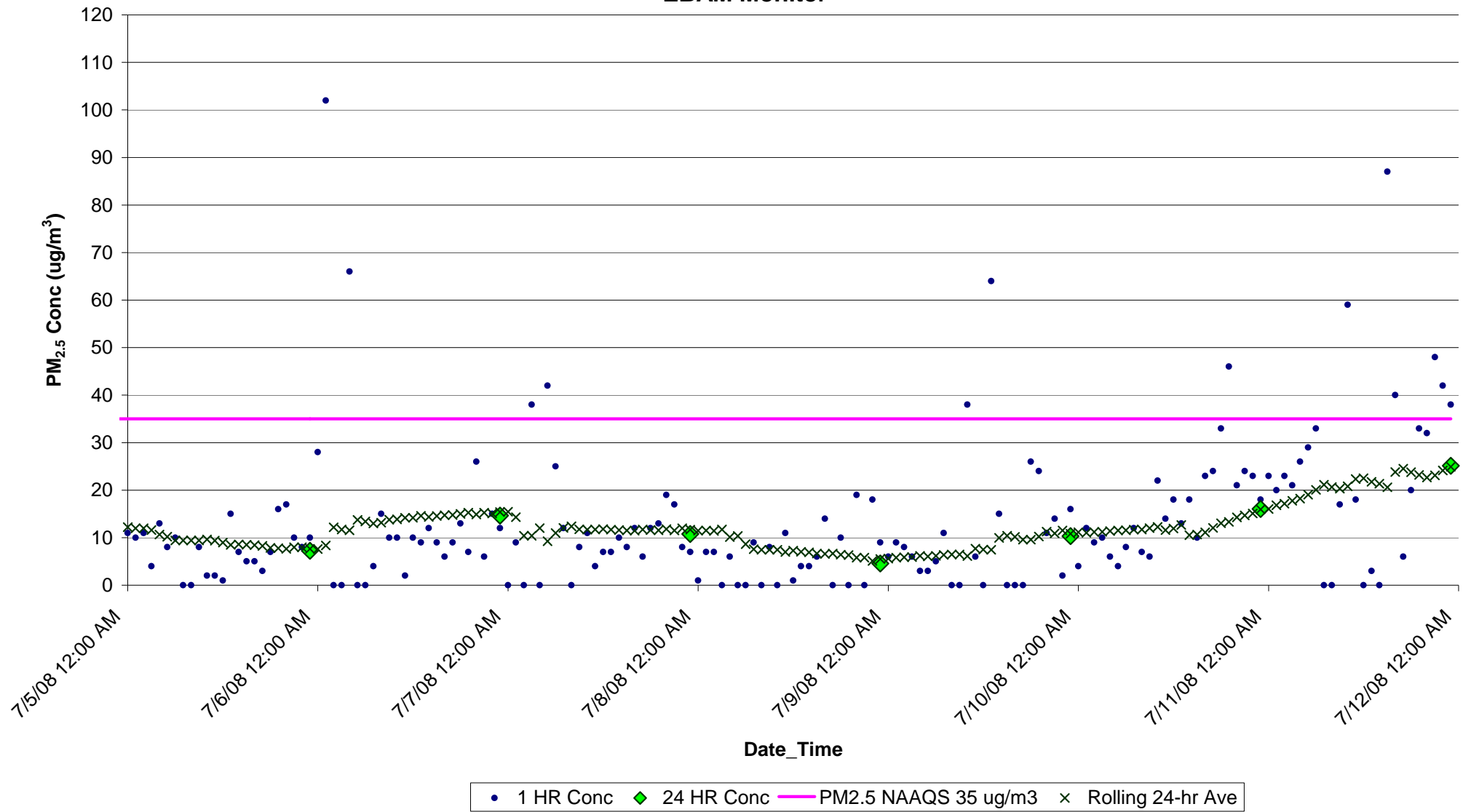
Figure F18. PM 2.5 Concentrations (ug/m 3 ) from July 5-11, 2008 for Fairfield, NC EBAM Monitor
