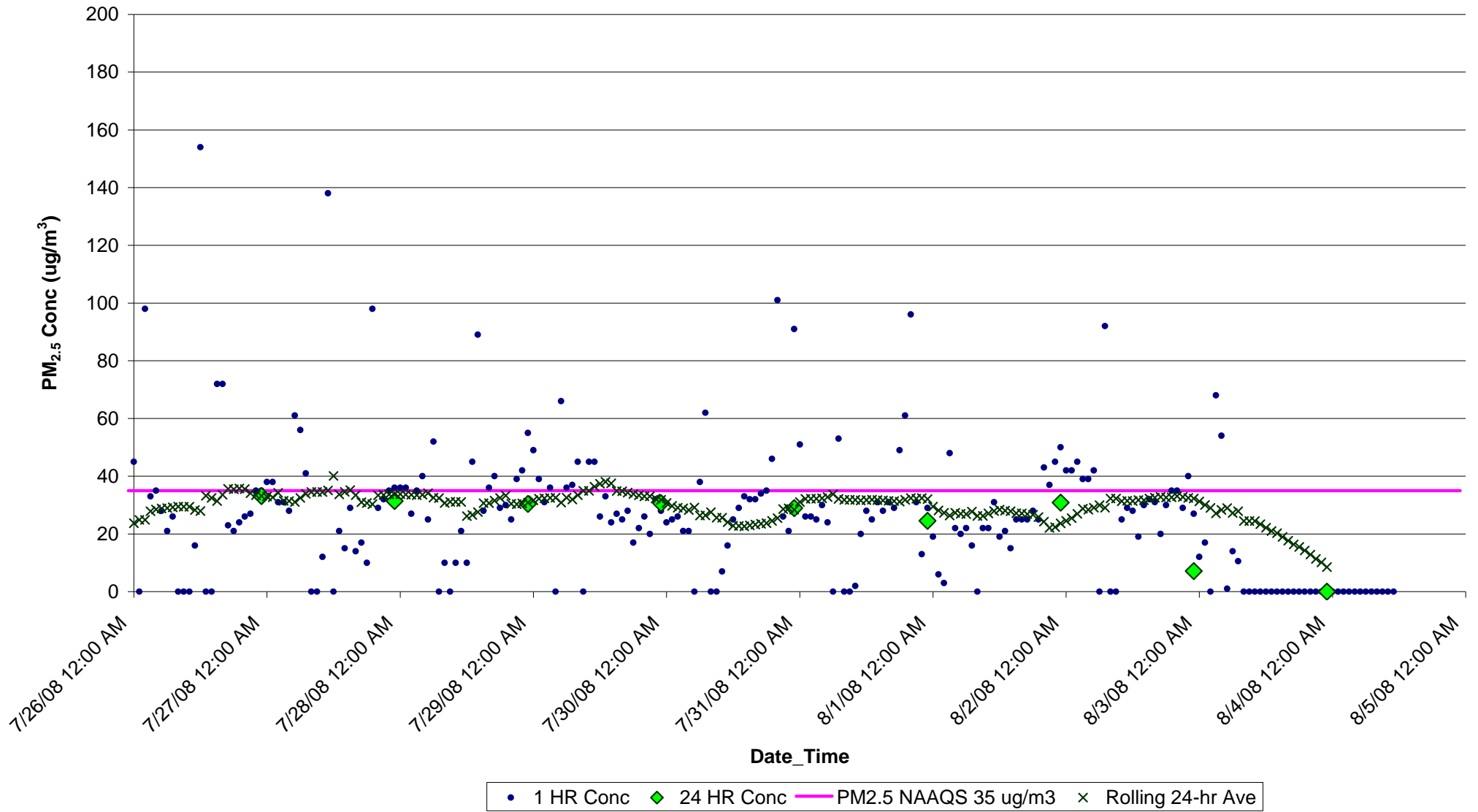
Figure F14. PM 2.5 Concentrations (ug/m 3 ) for July 26-Aug 4, 2008 at Columbia, NC EBAM Monitor
