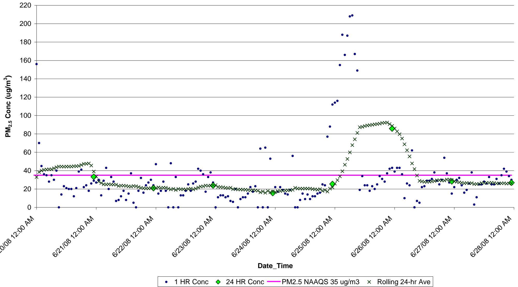
Figure F30. PM 2.5 Concentration (ug/m 3 ) from June 20-27, 2008 for Plymouth, NC EBAM Monitor
