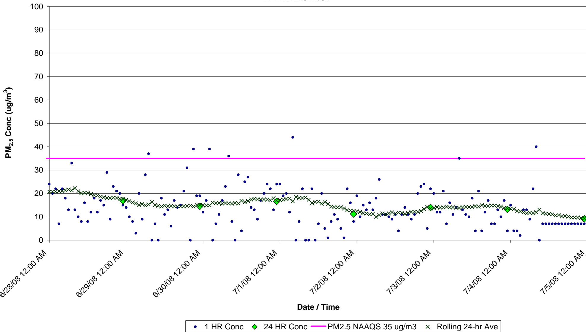
Figure F3. PM 2.5 Concentrations (ug/m 3 ) for June 28-July 4, 2008 at Belhaven, NC EBAM Monitor
