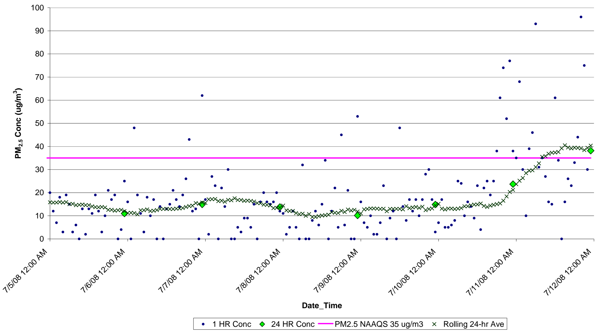
Figure F32. PM 2.5 Concentration (ug/m 3 ) from July 5-11, 2008 for Plymouth, NC EBAM Monitor
