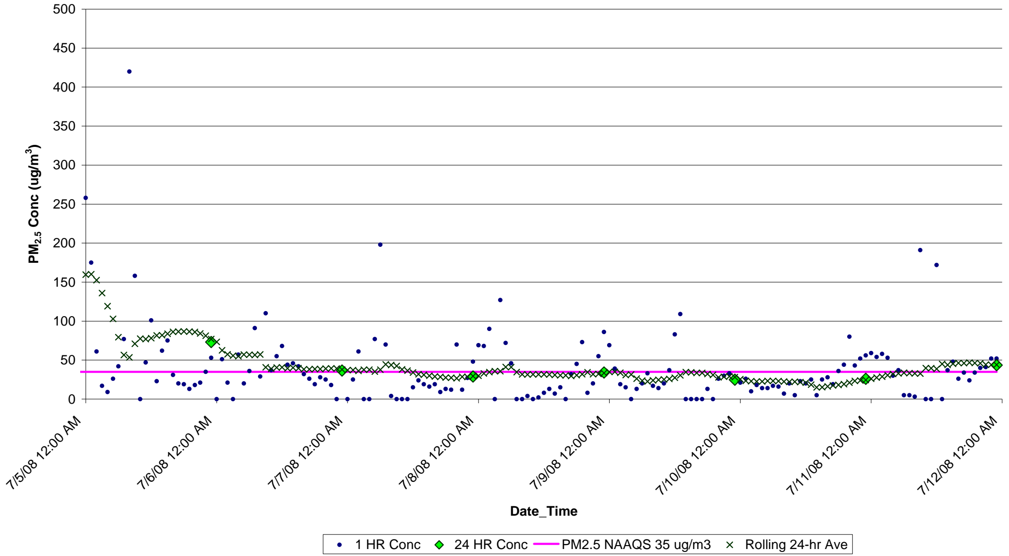
Figure F11. PM 2.5 Concentrations (ug/m 3 ) for July 5-11, 2008 at Columbia, NC EBAM Monitor
