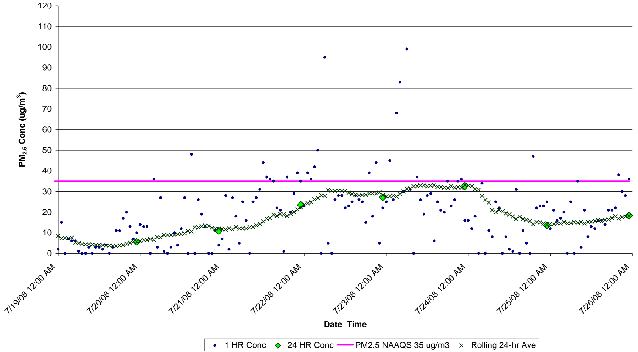
Figure F20. PM 2.5 Concentrations (ug/m 3 ) from July 19-25, 2008 for Fairfield, NC EBAM Monitor
