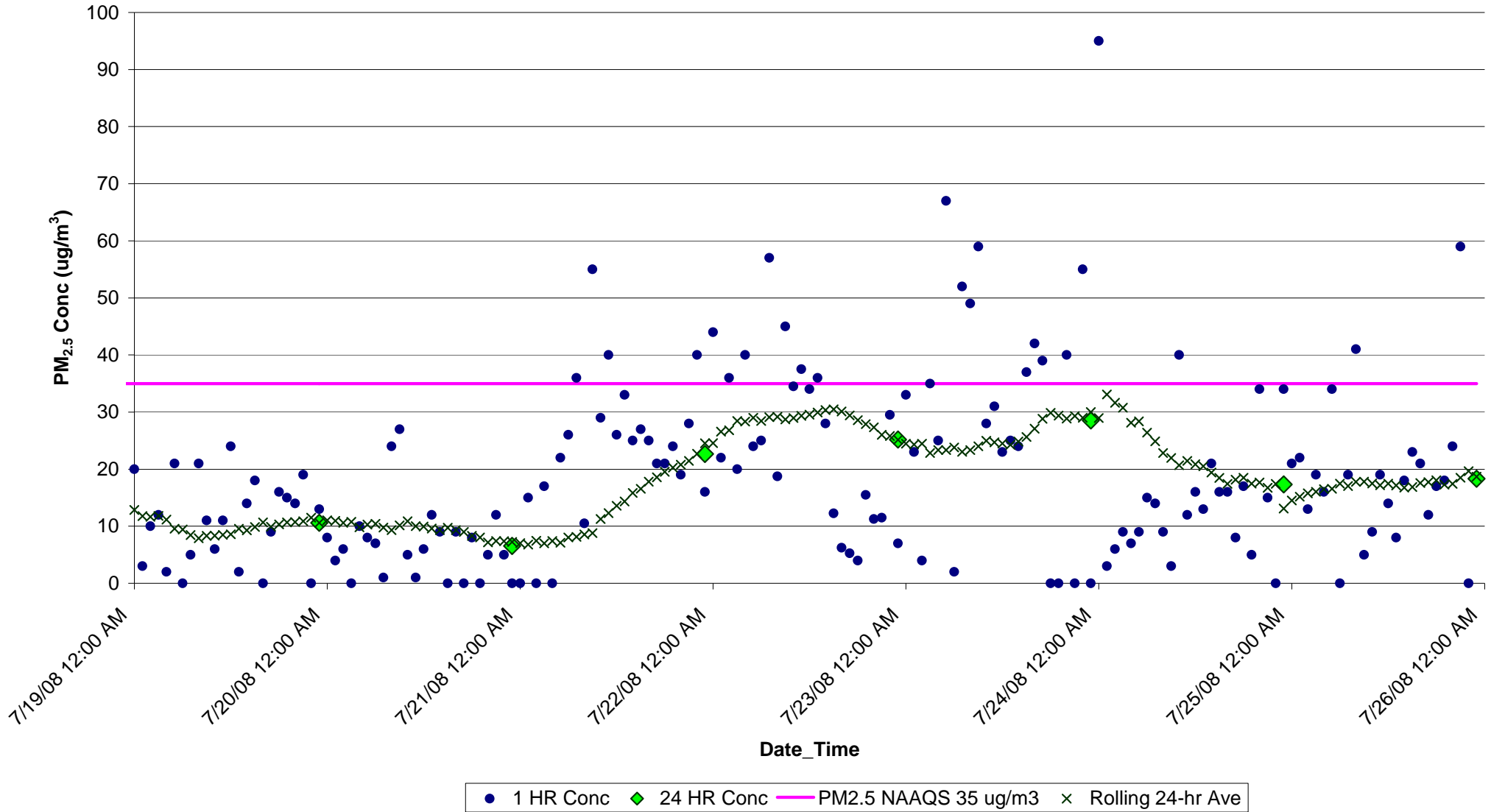
Figure F41. PM 2.5 Concentrations (ug/m 3 ) from July 19-25, 2008 for Washington, NC EBAM Monitor
