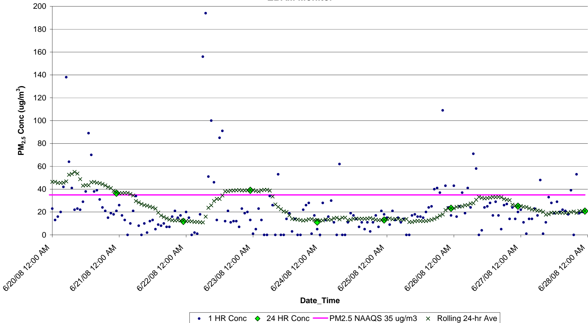
Figure F23. PM 2.5 Concentrations (ug/m 3 ) from June 20-27, 2008 for Manteo, NC EBAM Monitor
