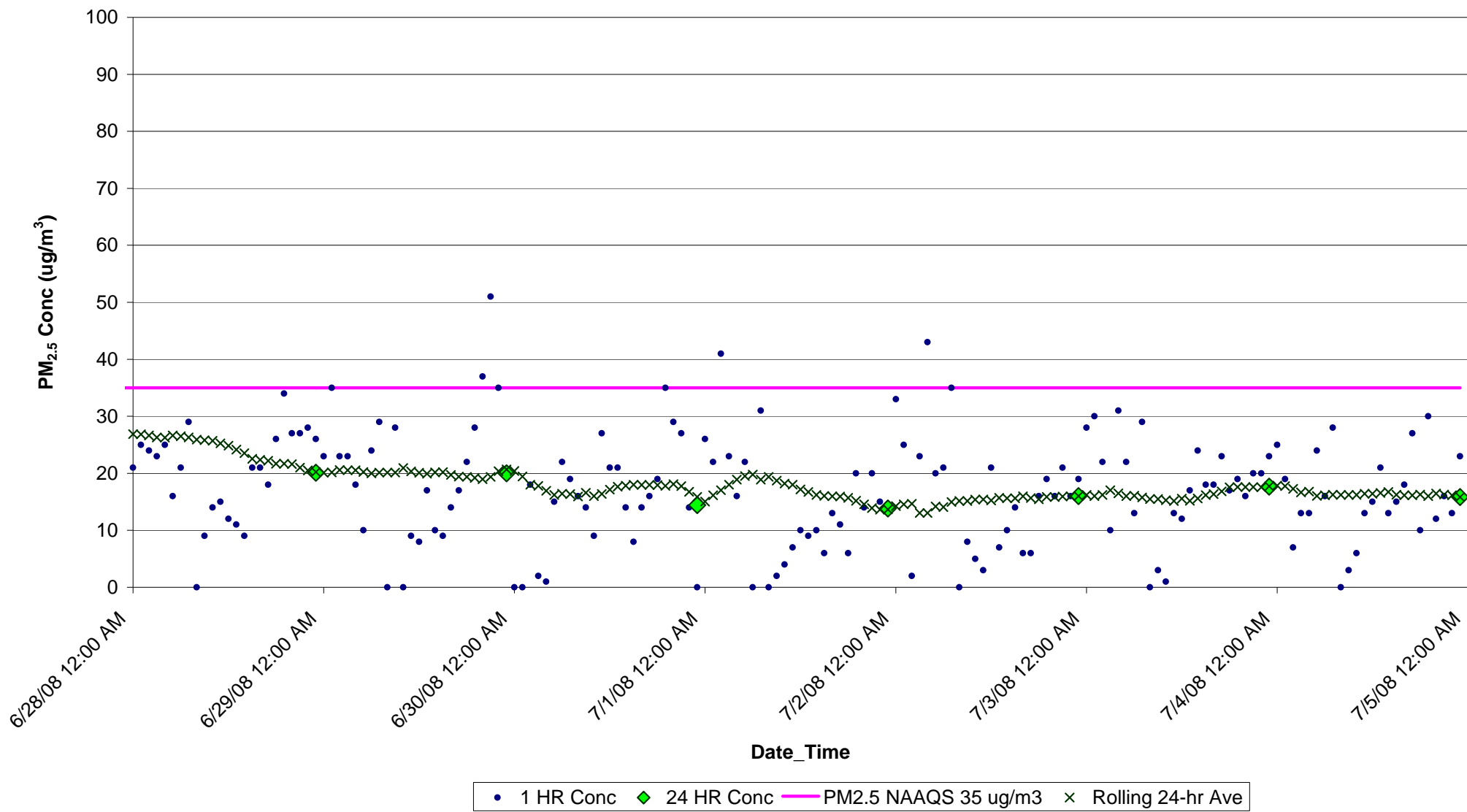
Figure F31. PM 2.5 Concentration (ug/m 3 ) from June 28-July 4, 2008 for Plymouth, NC EBAM Monitor
