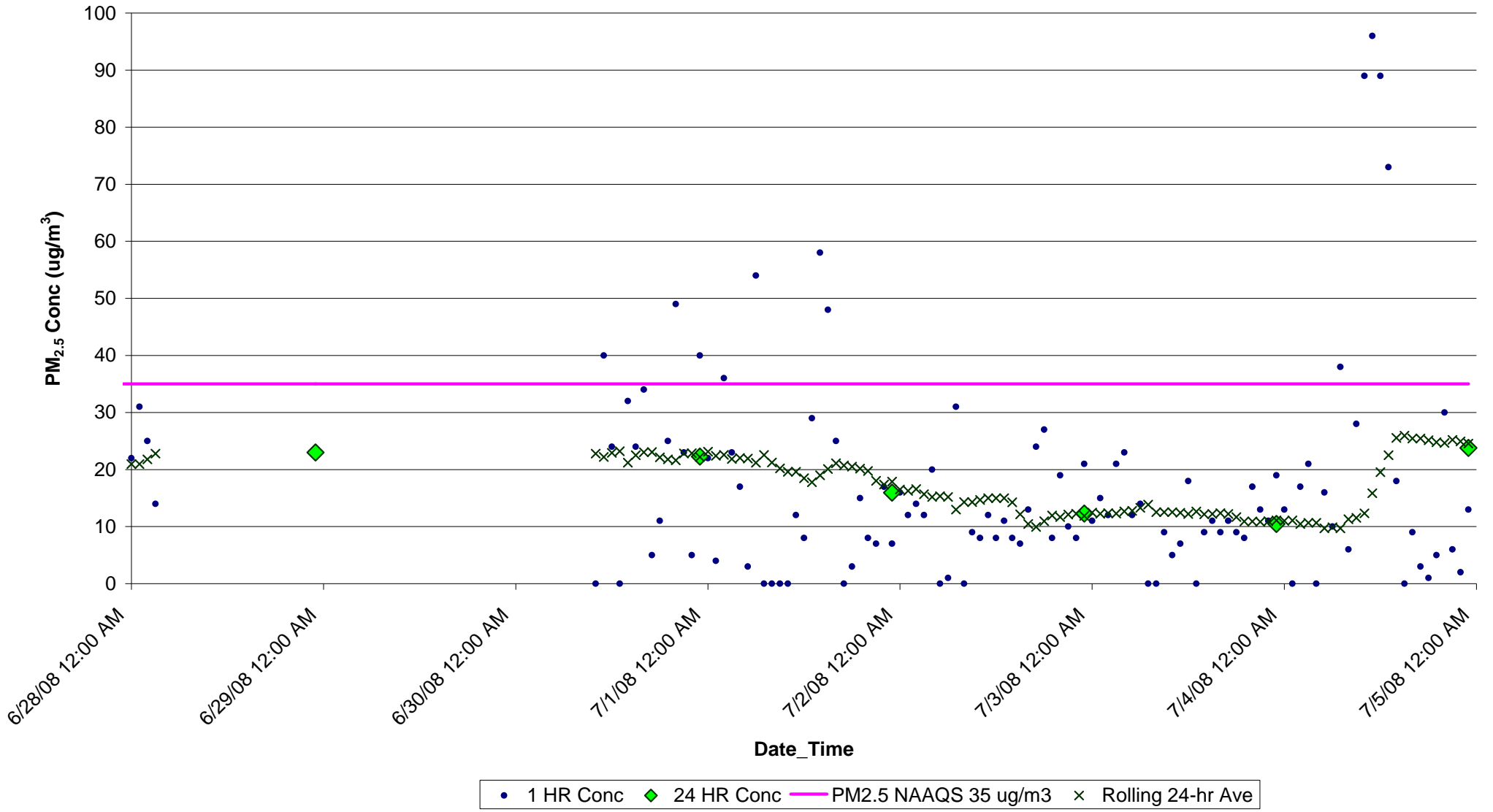
Figure F24. PM 2.5 Concentrations (ug/m 3 ) from June 28-July 4, 2008 for Manteo, NC EBAM Monitor
