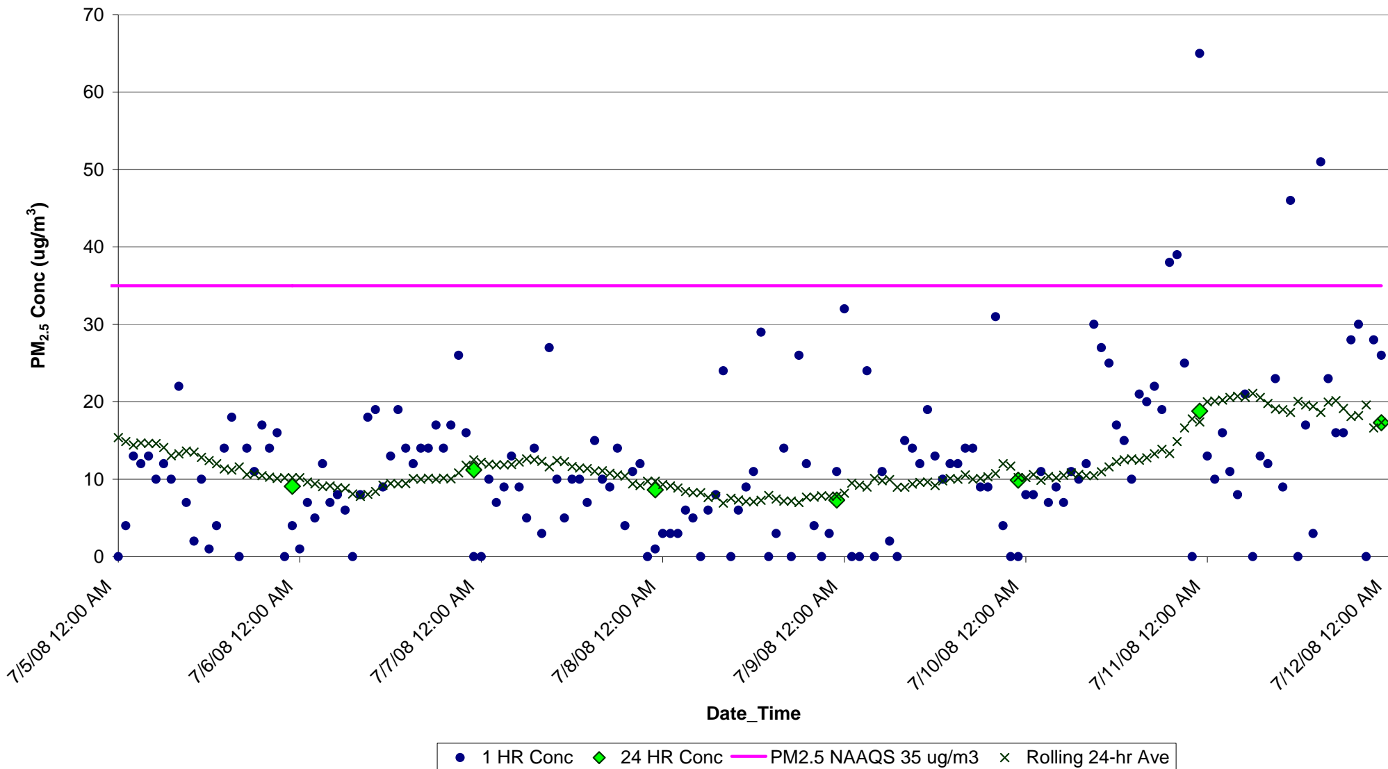
Figure F39. PM 2.5 Concentrations (ug/m 3 ) from July 5-11, 2008 for Washington, NC EBAM Monitor
