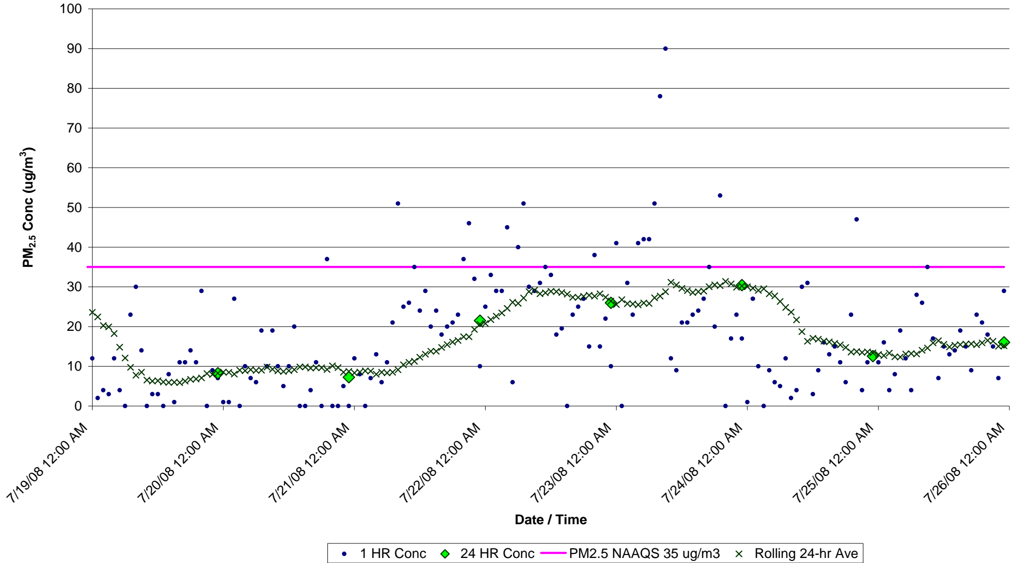
Figure F6. PM 2.5 Concentrations (ug/m 3 ) for July 19-25, 2008 at Belhaven, NC EBAM Monitor
