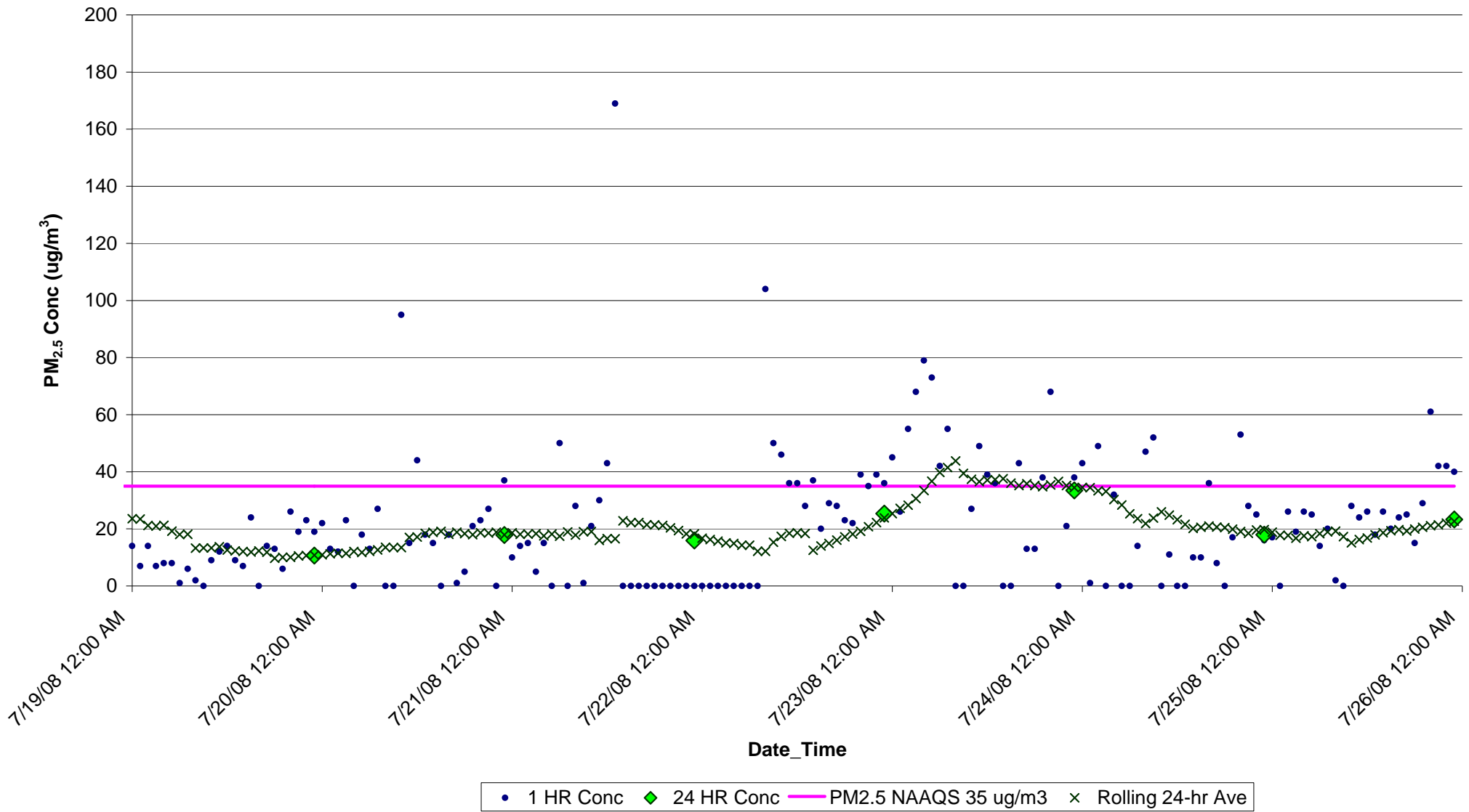
Figure F13. PM 2.5 Concentrations (ug/m 3 ) for July 19-25, 2008 at Columbia, NC EBAM Monitor
