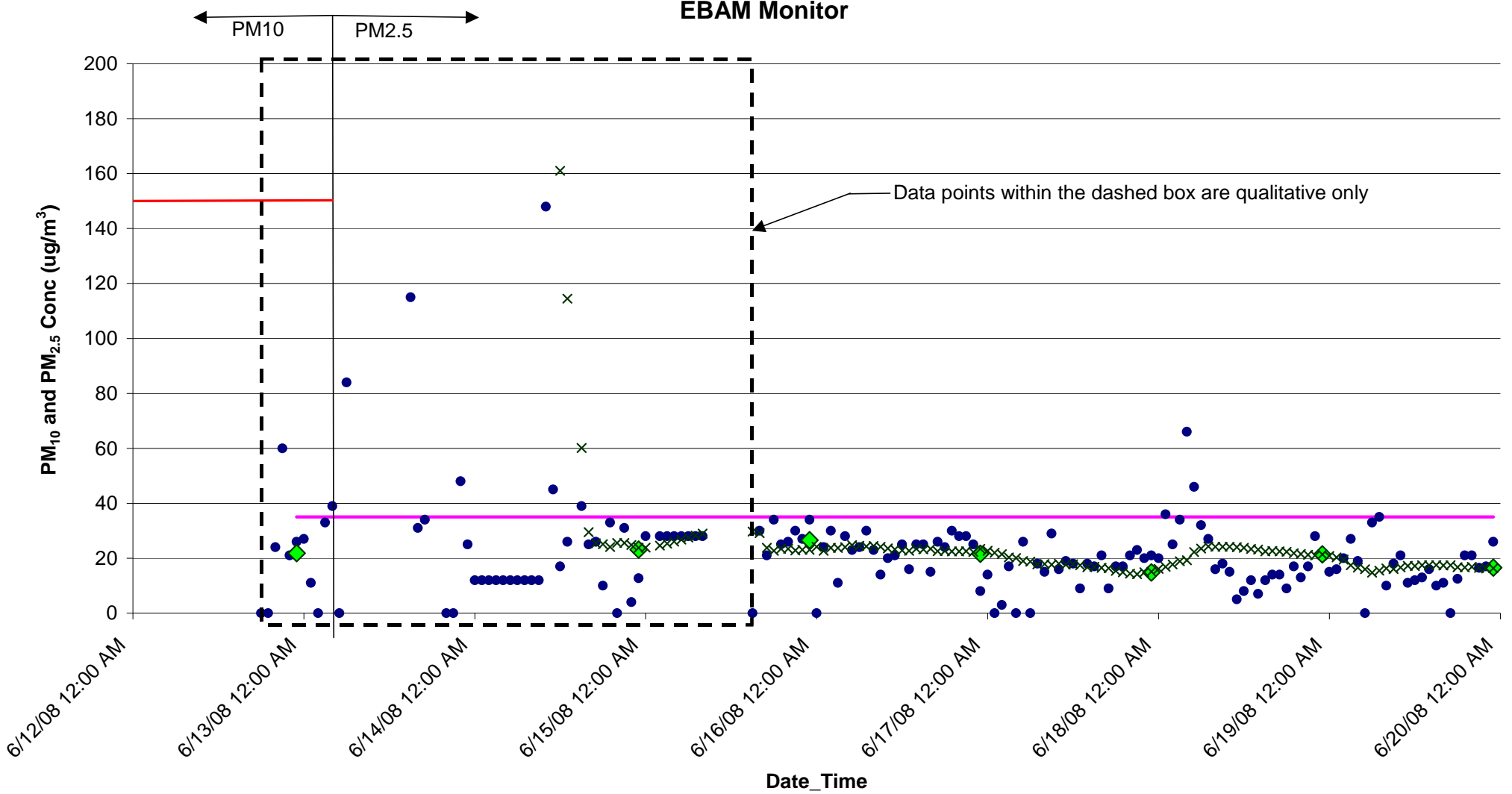
Figure F36a. PM 10 and PM 2.5 Concentrations (ug/m 3 ) from June 12-19, 2008 for Washington, NC
