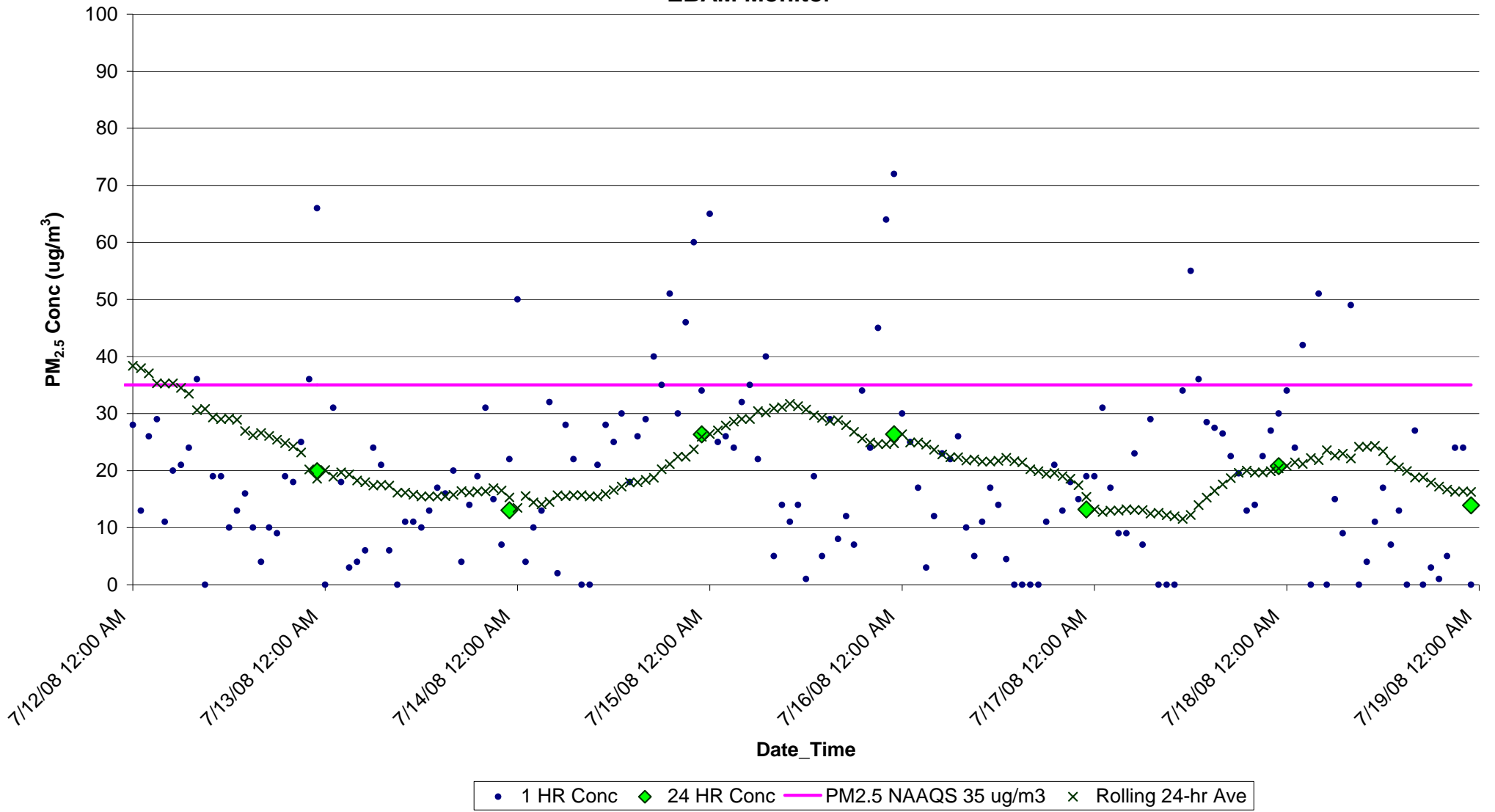
Figure F33. PM 2.5 Concentration (ug/m 3 ) from July 12-18, 2008 for Plymouth, NC EBAM Monitor
