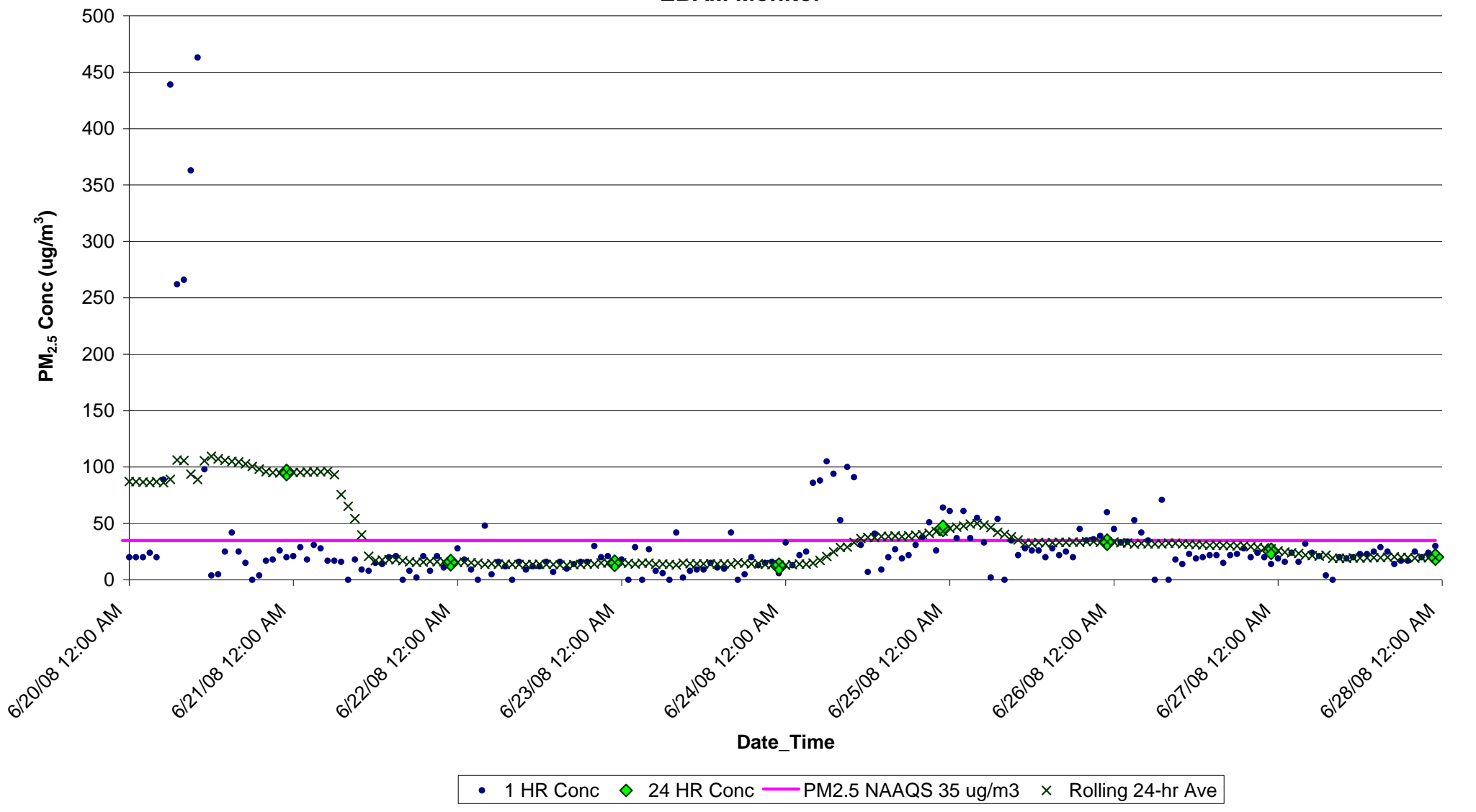
Figure F16. PM 2.5 Concentrations (ug/m 3 ) from June 20-27, 2008 for Fairfield, NC EBAM Monitor
