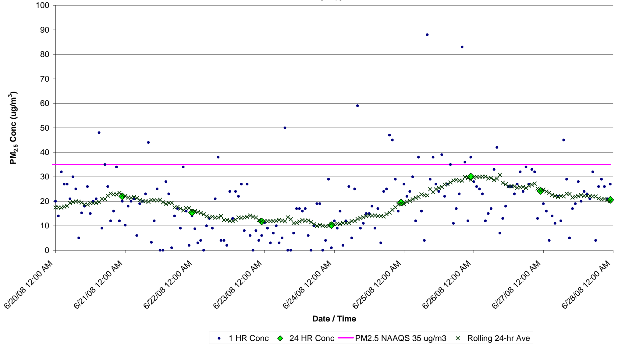
Figure F2. PM 2.5 Concentrations (ug/m 3 ) for June 20-27, 2008 at Belhaven, NC EBAM Monitor
