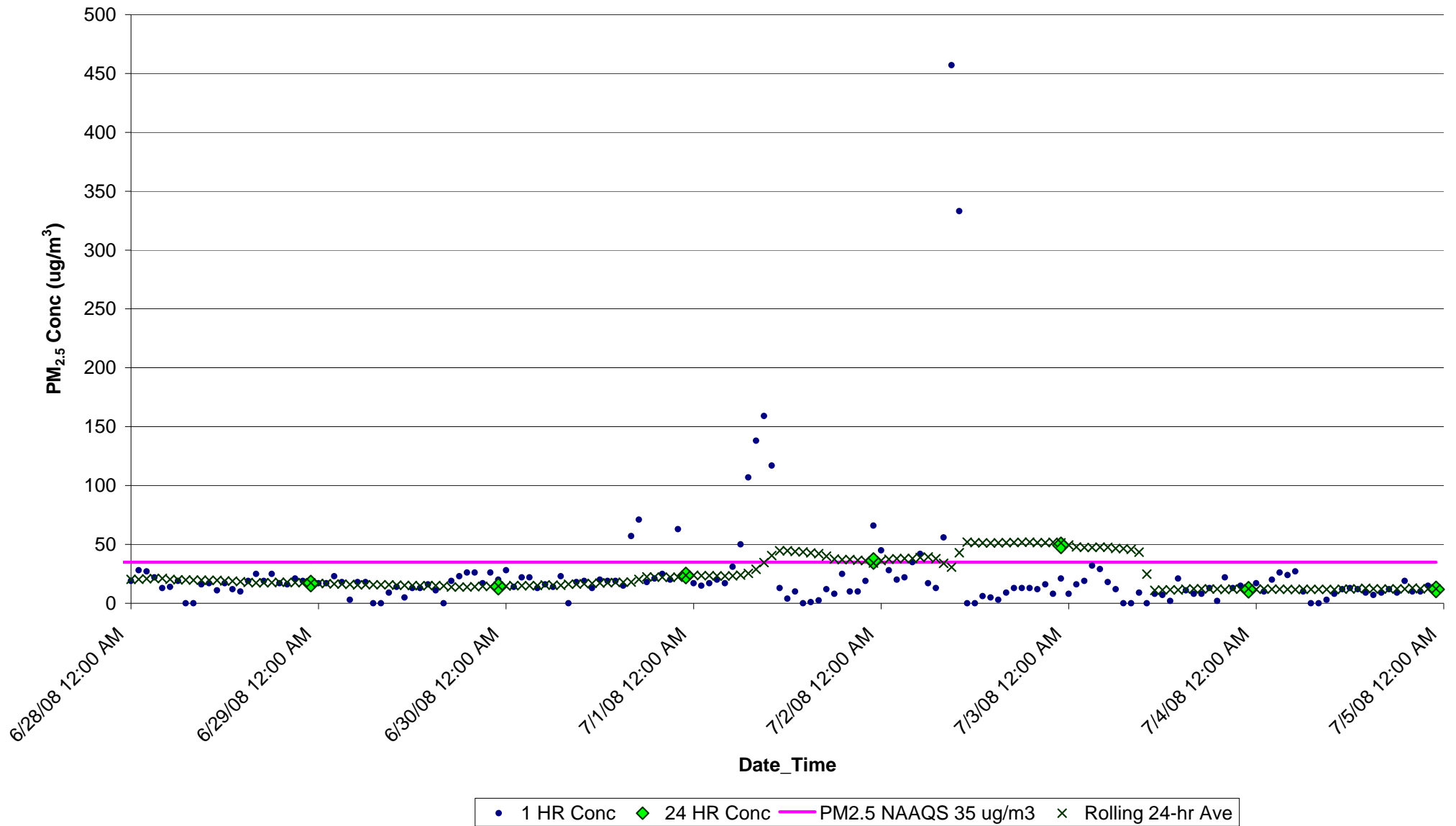
Figure F17. PM 2.5 Concentrations (ug/m 3 ) from June 28-July 4, 2008 for Fairfield, NC EBAM Monitor
