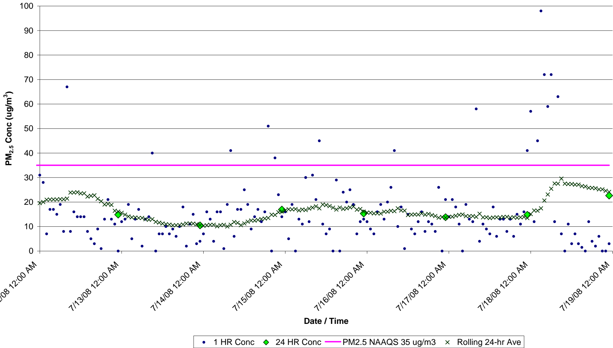
Figure F5. PM 2.5 Concentrations (ug/m 3 ) for July 12-18, 2008 at Belhaven, NC EBAM Monitor
