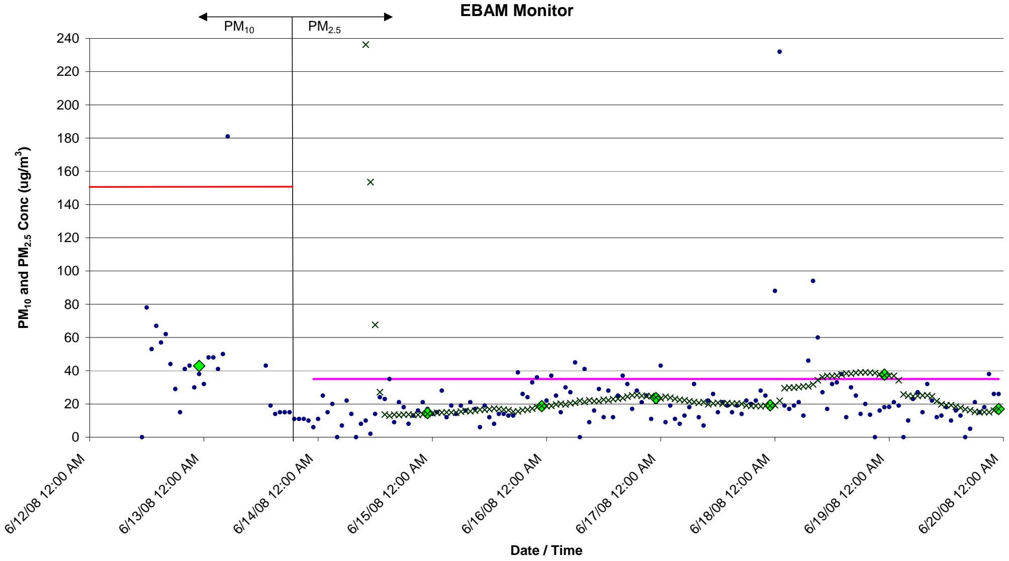
Figure F1a. PM 10 and PM 2.5 Concentrations (ug/m 3 ) for June 12-19, 2008 at Belhaven, NC
