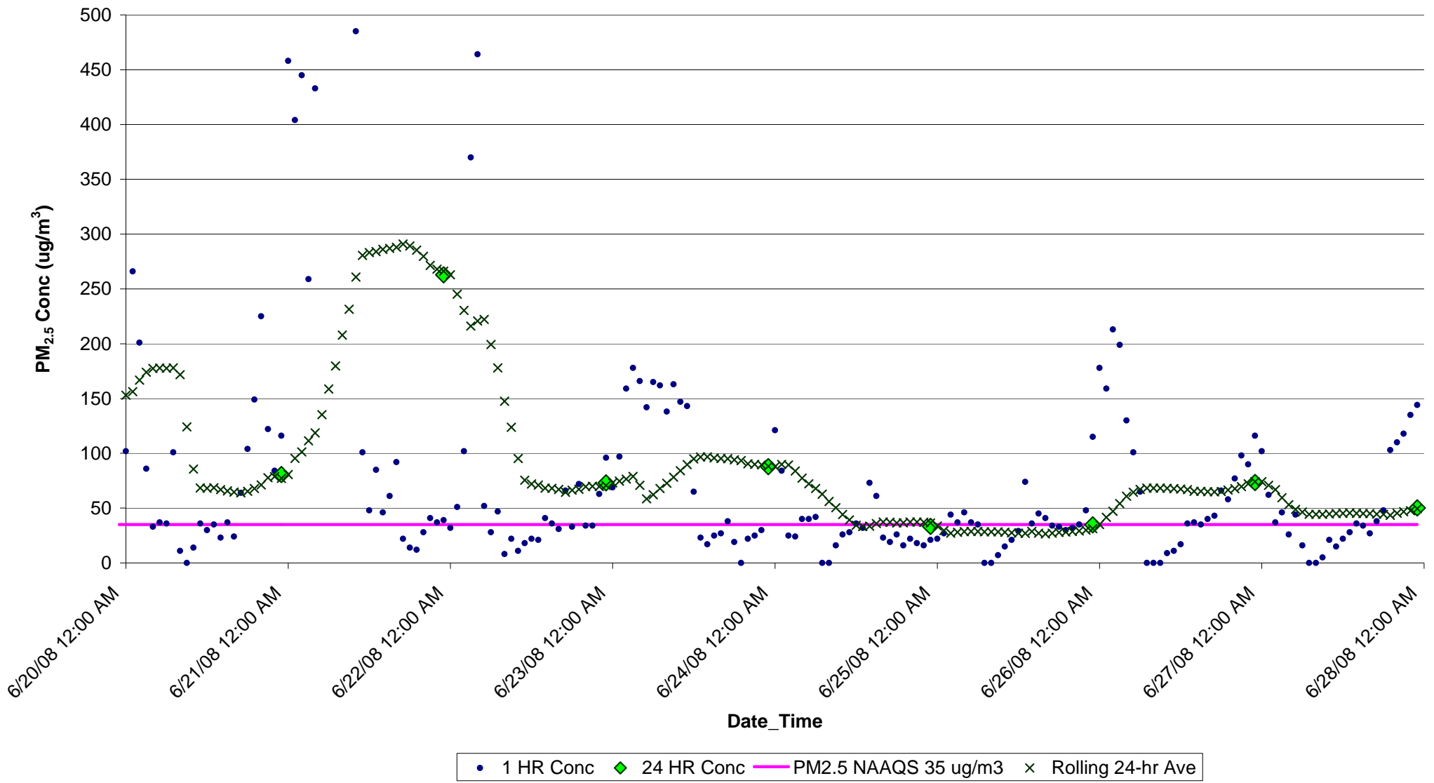
Figure F9. PM 2.5 Concentrations (ug/m 3 ) for June 20-27, 2008 at Columbia, NC EBAM Monitor
