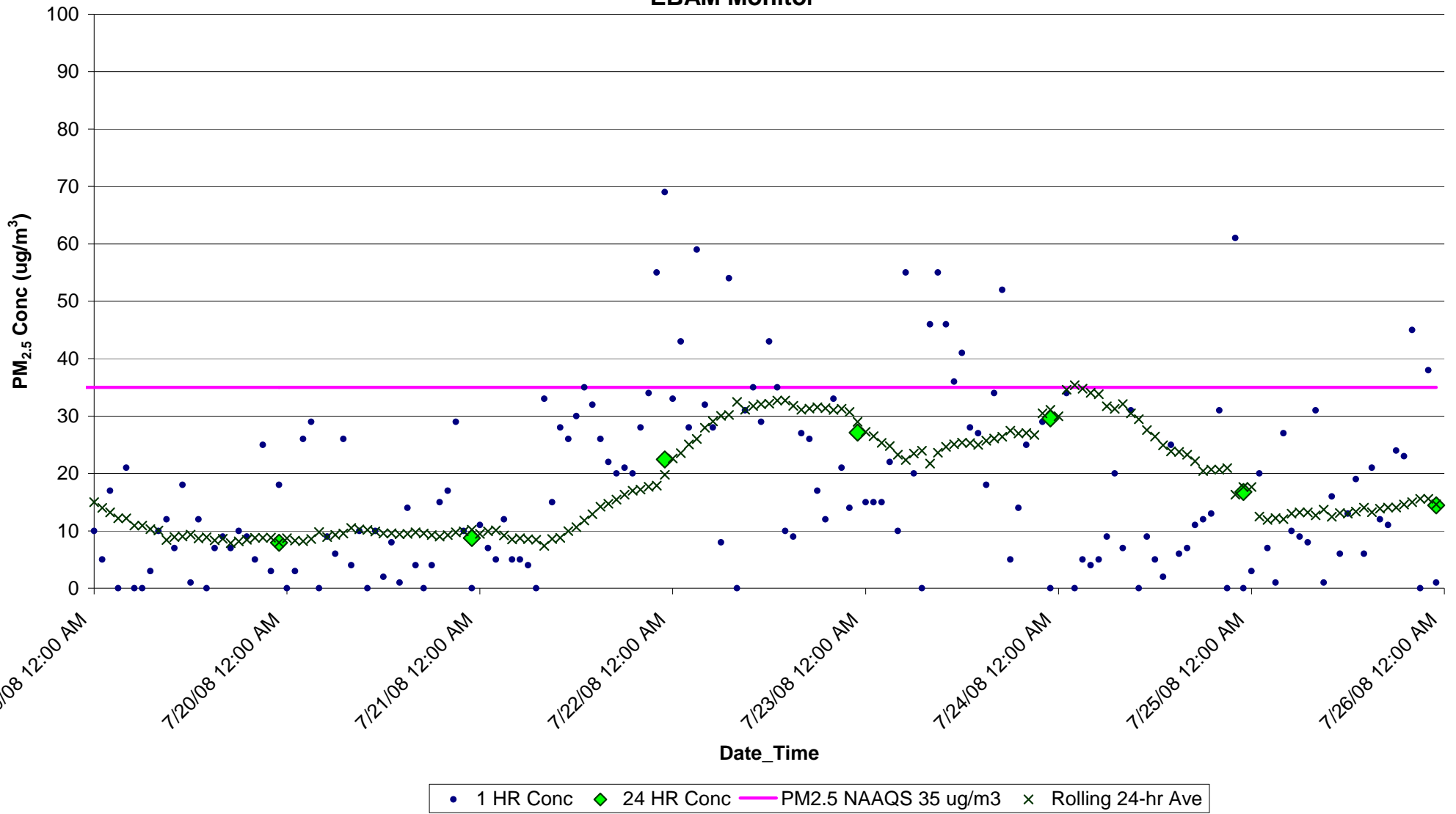
Figure F34. PM 2.5 Concentration (ug/m 3 ) from July 19-25, 2008 for Plymouth, NC EBAM Monitor
