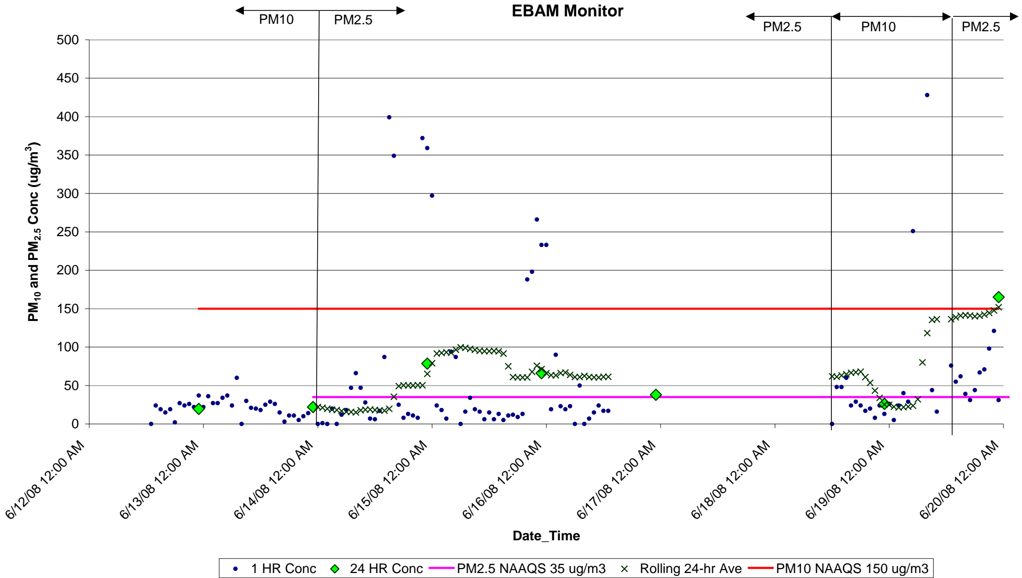
Figure F8. PM 10 and PM 2.5 Concentrations (ug/m 3 ) for June 12-19, 2008 at Columbia, NC
