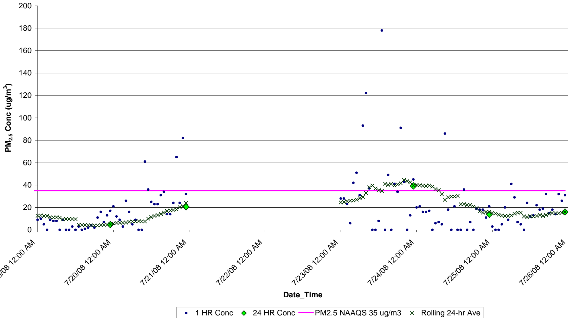
Figure F27. PM 2.5 Concentrations (ug/m 3 ) from July 19-25, 2008 for Manteo, NC EBAM Monitor
