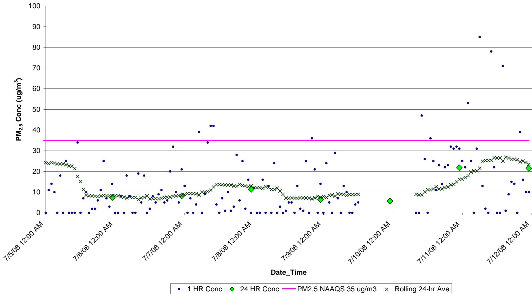
Figure F25. PM 2.5 Concentrations (ug/m 3 ) from July 5-11, 2008 for Manteo, NC EBAM Monitor
