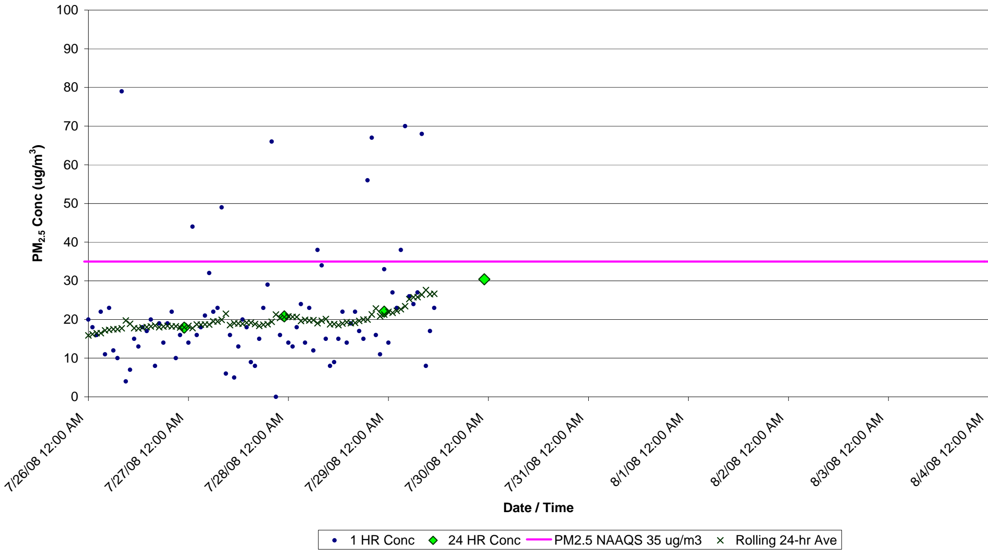
Figure F7. PM 2.5 Concentrations (ug/m 3 ) for July 26-Aug 4, 2008 at Belhaven, NC EBAM Monitor
