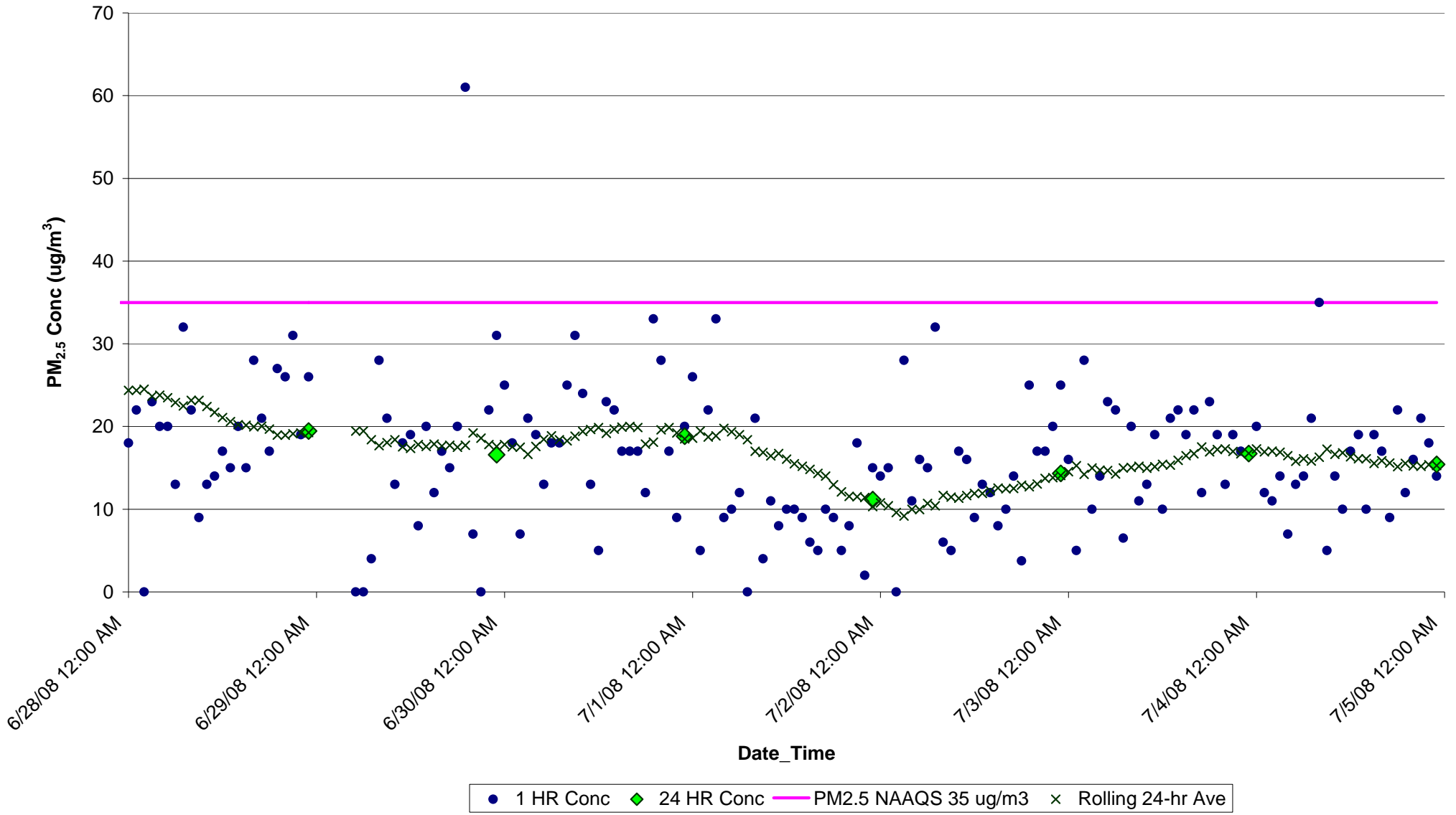
Figure F38. PM 2.5 Concentrations (ug/m 3 ) from June 28-July 4, 2008 for Washington, NC EBAM Monitor
