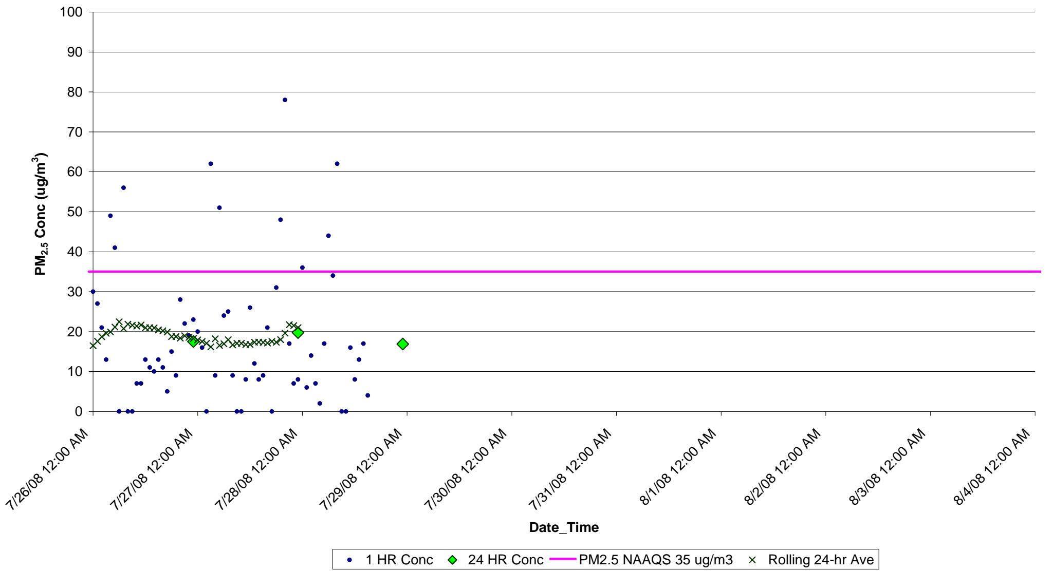
Figure F28. PM 2.5 Concentrations (ug/m 3 ) from July 26-Aug 4, 2008 for Manteo, NC EBAM Monitor
