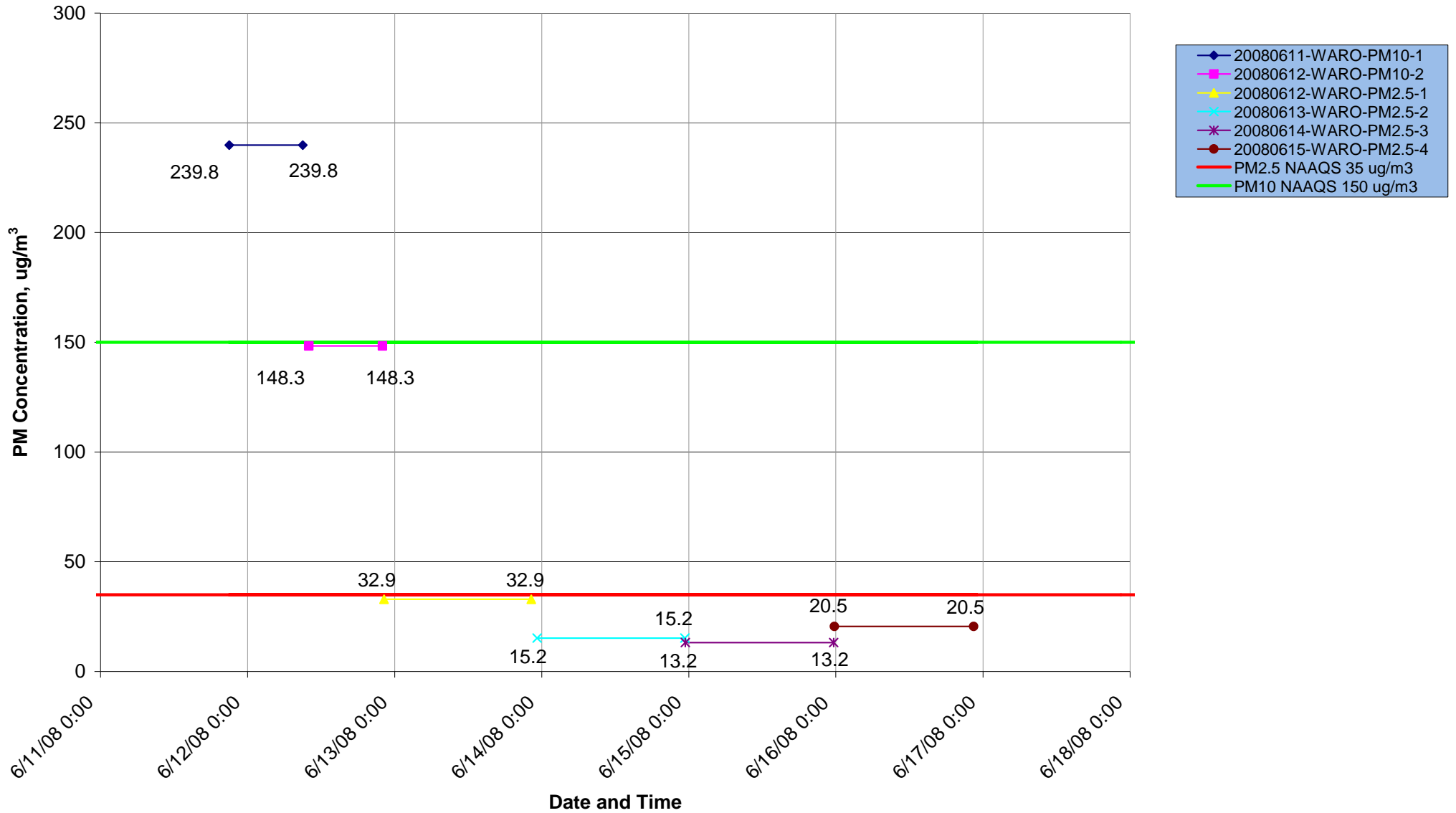
Figure D1. PM 10 and PM 2.5 Concentrations (ug/m 3 ) for June 11-18, 2008 at Washington, NC OMNI Monitor
