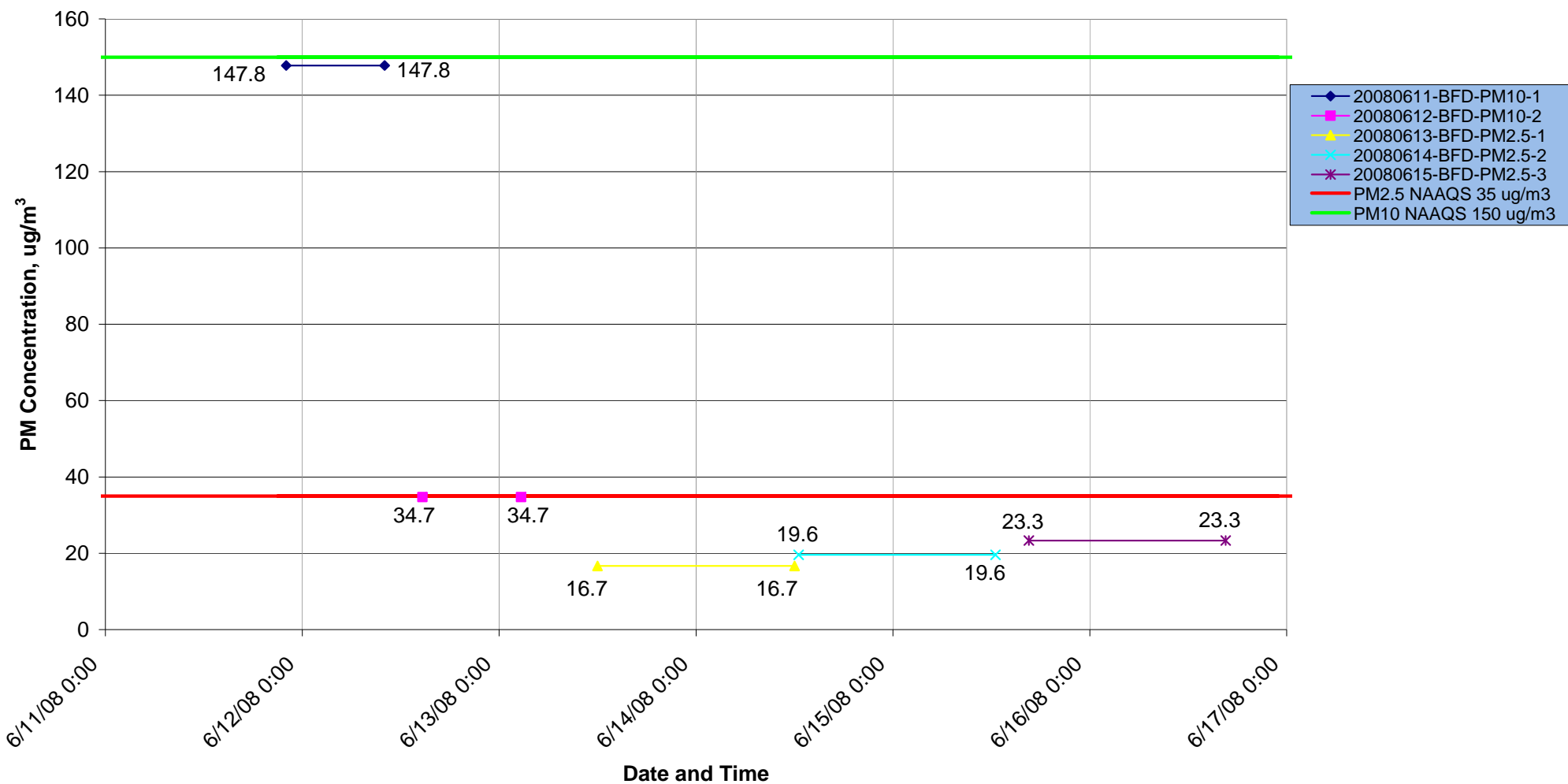
Figure D2. PM 10 and PM 2.5 Concentrations (ug/m 3 ) for June 11-17, 2008 at Belhaven, NC OMNI Monitor
