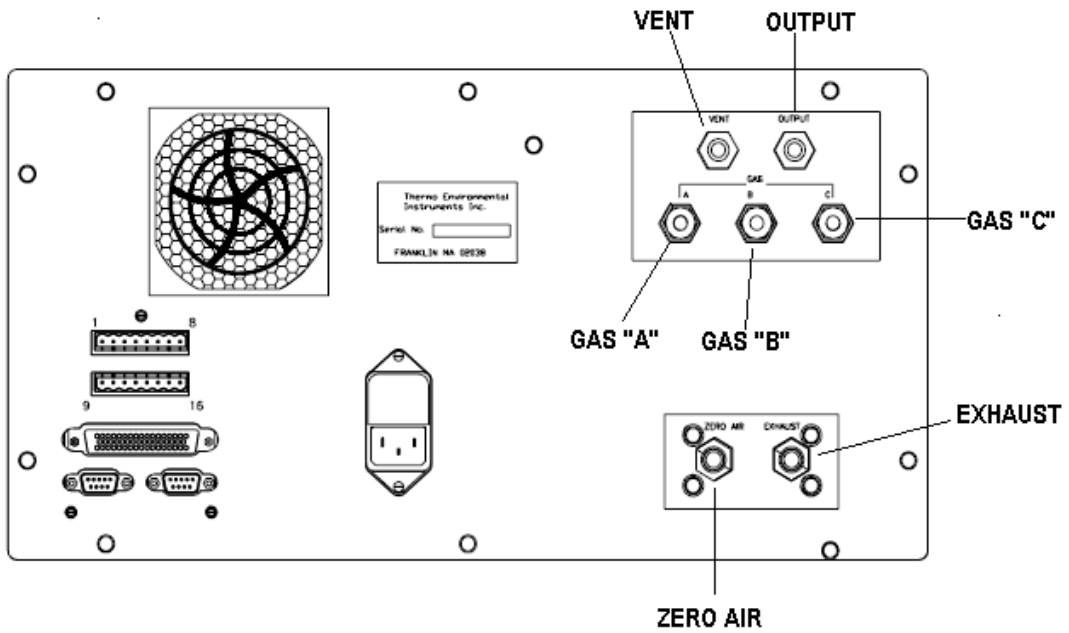
Figure 3 146C Rear View
