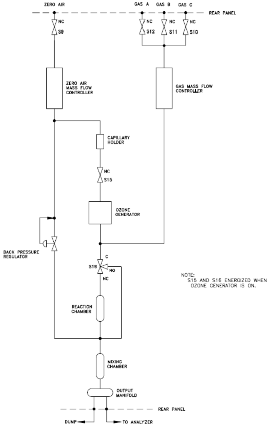
Figure 1 Model 146C Hardware Configuration, Standard Gas Dilution System
